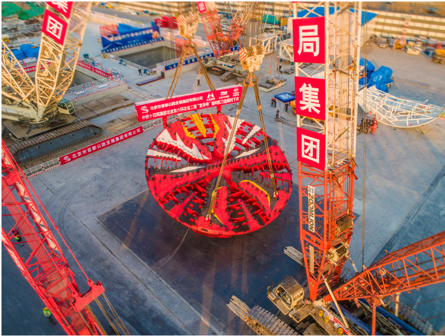
Φ16.07m slurry TBM applied in Beijing East 6th Ring Road Tunnel, China. Max. monthly advance rate 542 meters was achieved.
